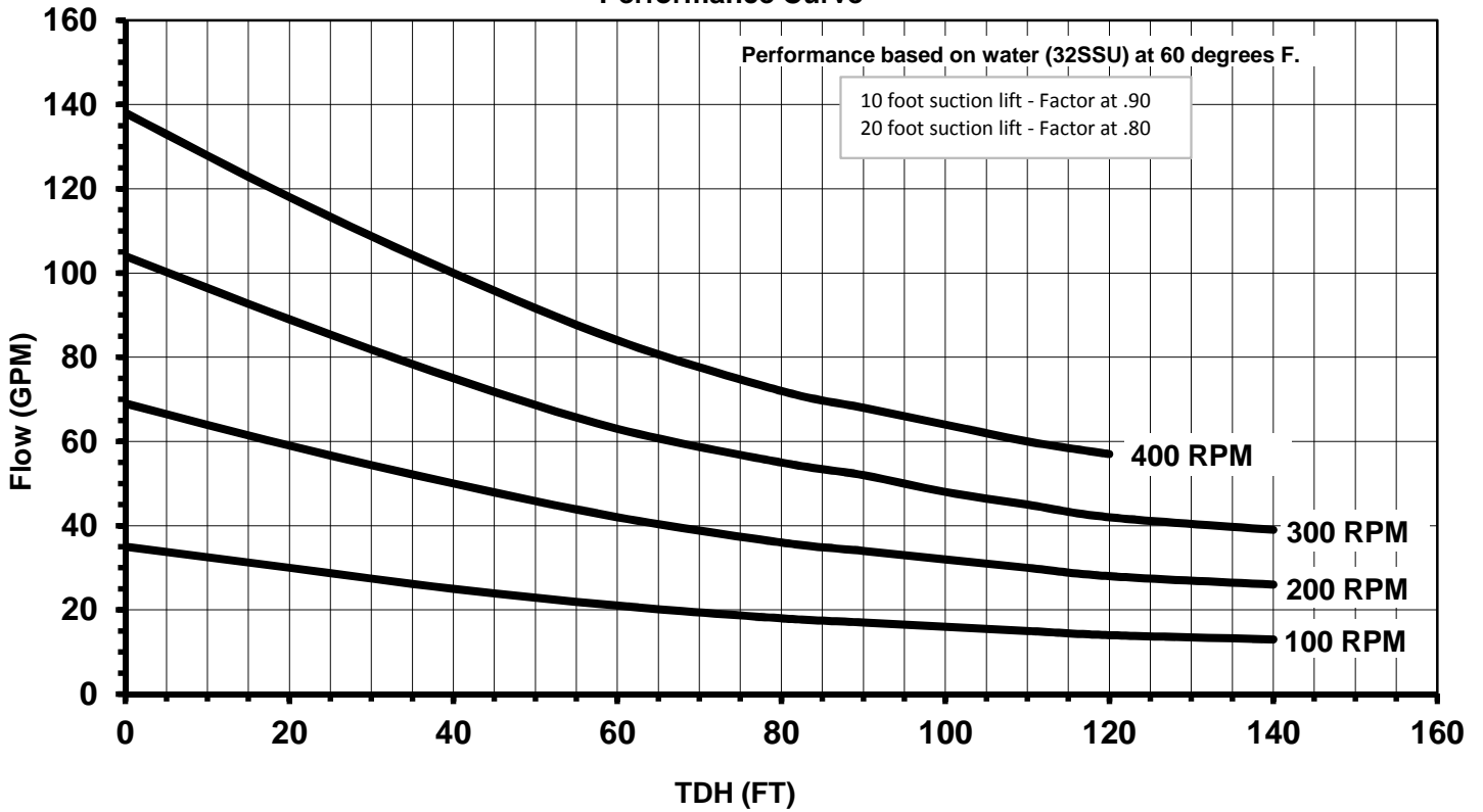
Performance Curve
